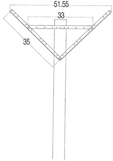
Pipe End Post with the Small End V Assembly
